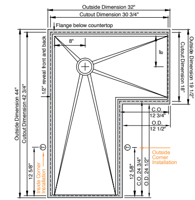
Center Galley Tap holes 2" from the back of the 18" countertop cutout
