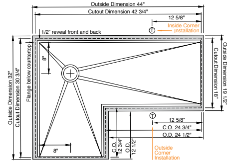
Center Galley Tap holes 2" from the back of the 18" countertop cutout
