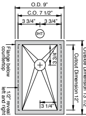
Center Galley Tap hole 2" from the back of the 12" countertop cutout
