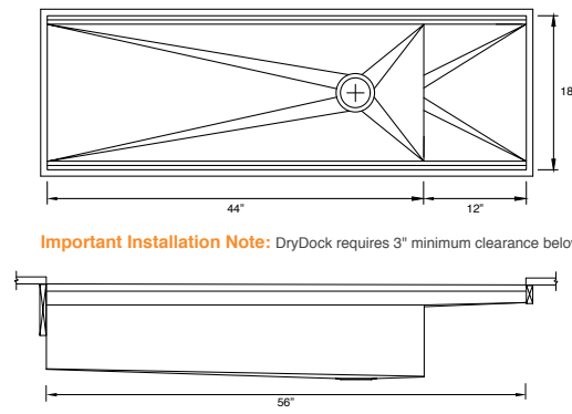
IWS-4-S-DD-12-S-TT-xx
