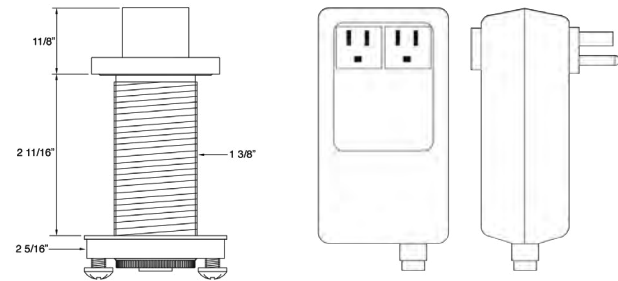
Appliance Control Box 4 3/8" H x 3" W x 1 3/4" D 120v 15amp 1Hp
