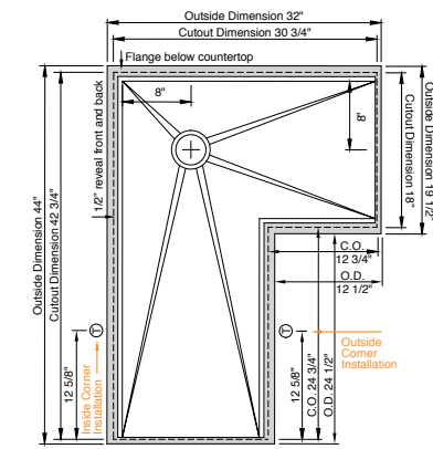
Center Galley Tap holes 2" from the back of the 18" countertop cutout
