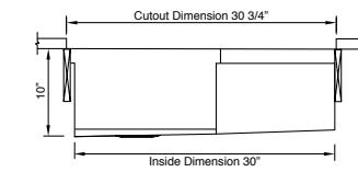
Center Galley Tap holes 2" from the back of the 18" countertop cutout
